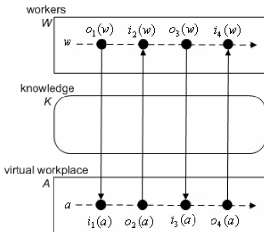
Figure 5. 2-Support relatedness
